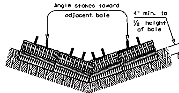
PROFILE VIEW
